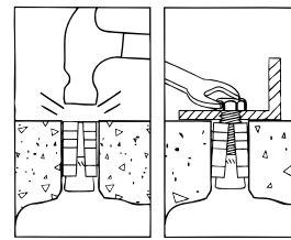
Drop-In Anchor
